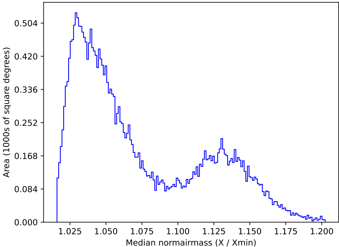
ddf_loaded_fl15_v3.4_10yrs All sky i band: Median normairmass
