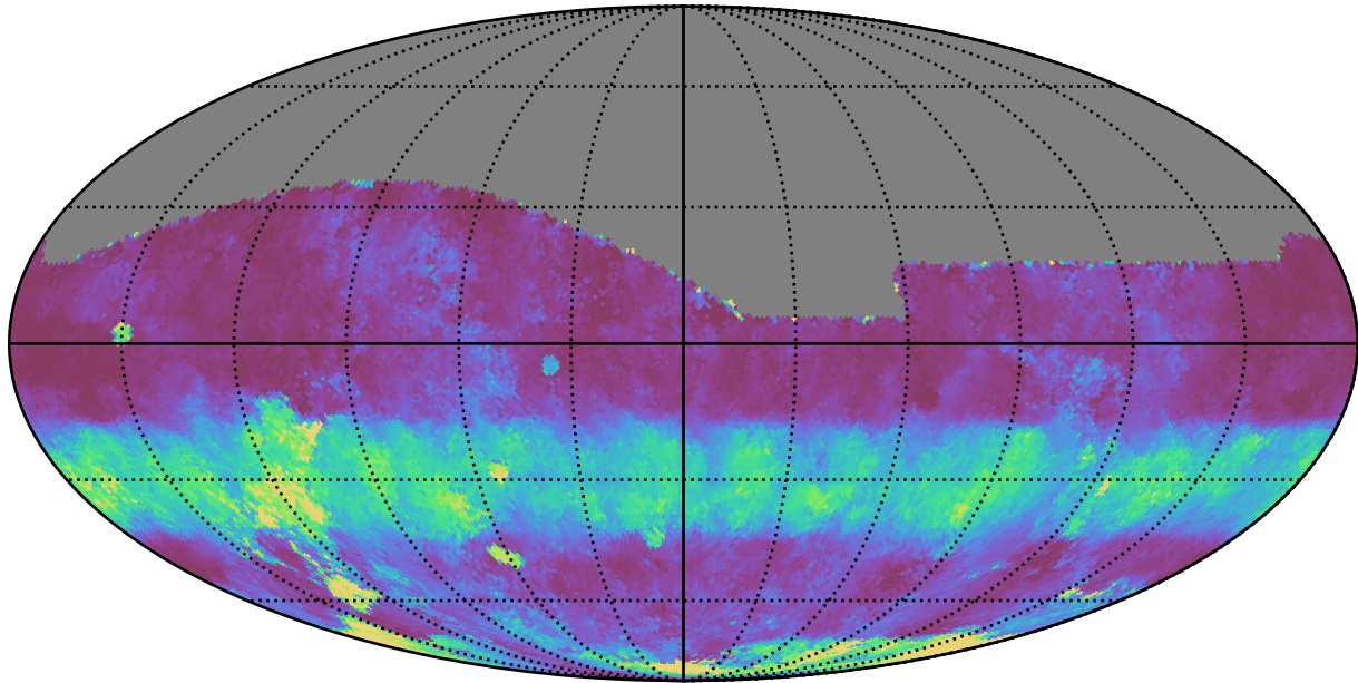
ddf_loaded_fl15_v3.4_10yrs All sky g band: Median normairmass
