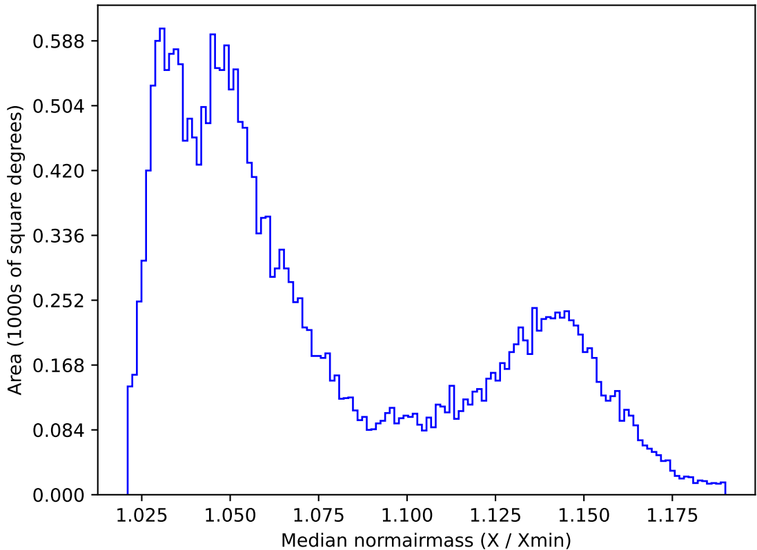
ddf_loaded_fl15_v3.4_10yrs All sky all bands: Median normairmass
