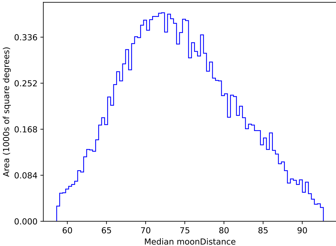
ddf_loaded_fl15_v3.4_10yrs WFD z band: Median moonDistance
