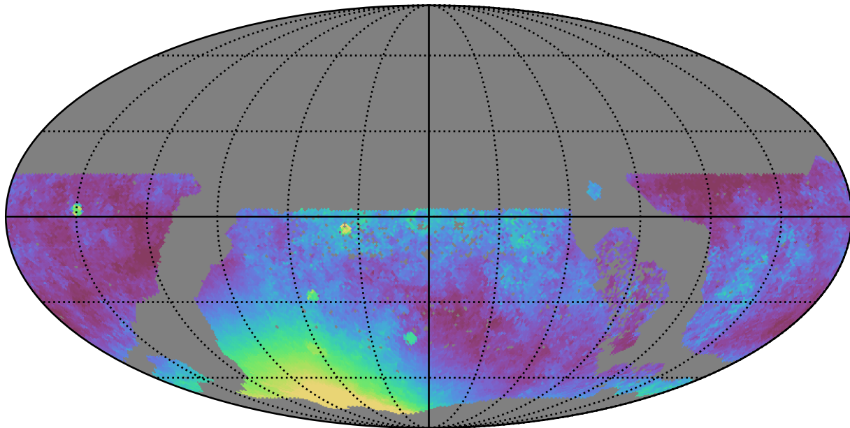
ddf_loaded_fl15_v3.4_10yrs WFD y band: Median moonDistance
