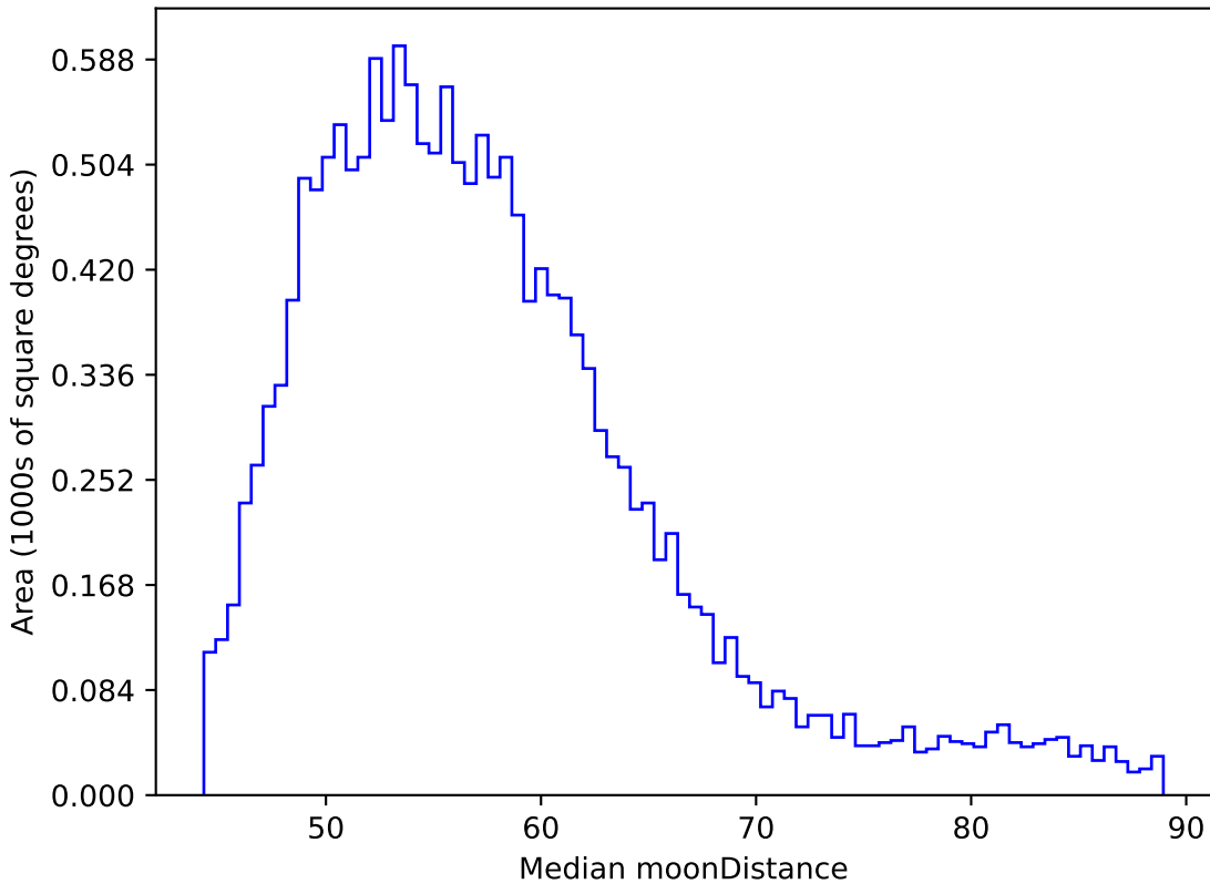
ddf_loaded_fl15_v3.4_10yrs WFD y band: Median moonDistance
