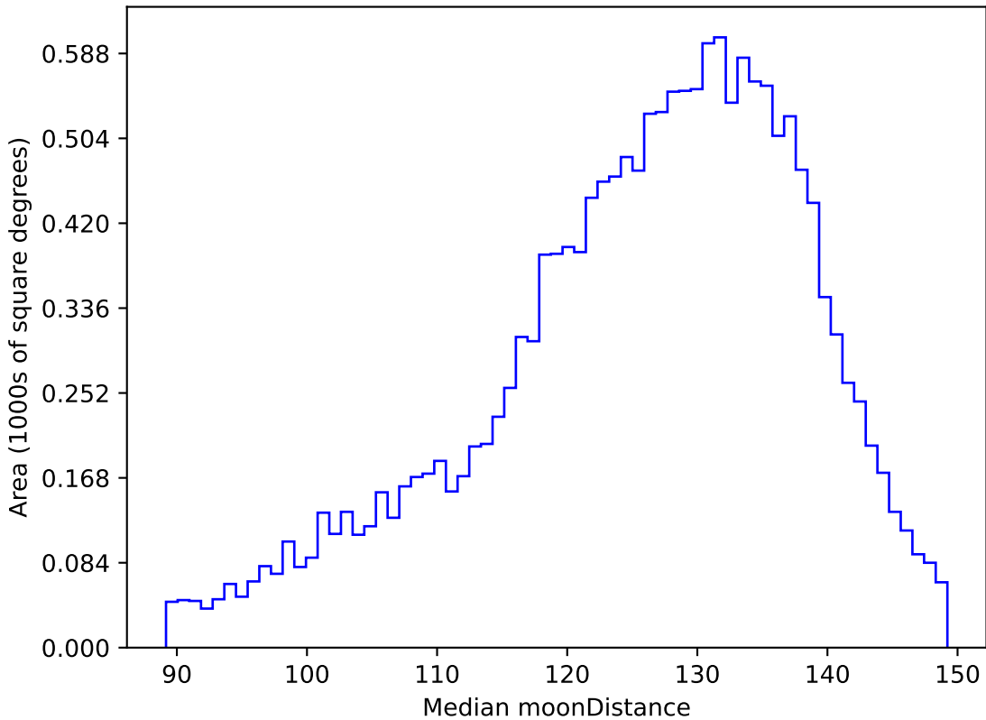
ddf_loaded_fl15_v3.4_10yrs WFD u band: Median moonDistance
