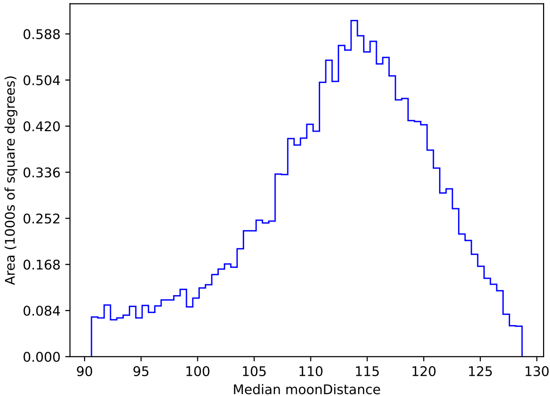
ddf_loaded_fl15_v3.4_10yrs WFD r band: Median moonDistance
