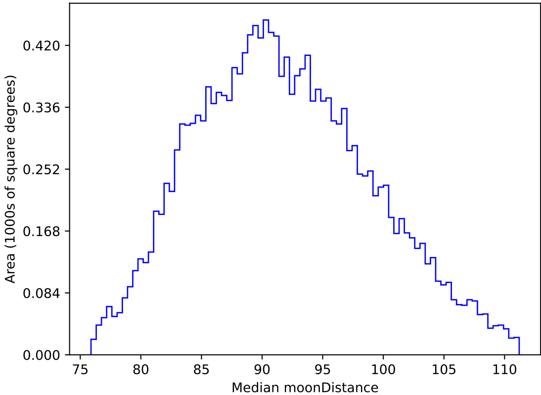
ddf_loaded_fl15_v3.4_10yrs WFD i band: Median moonDistance
