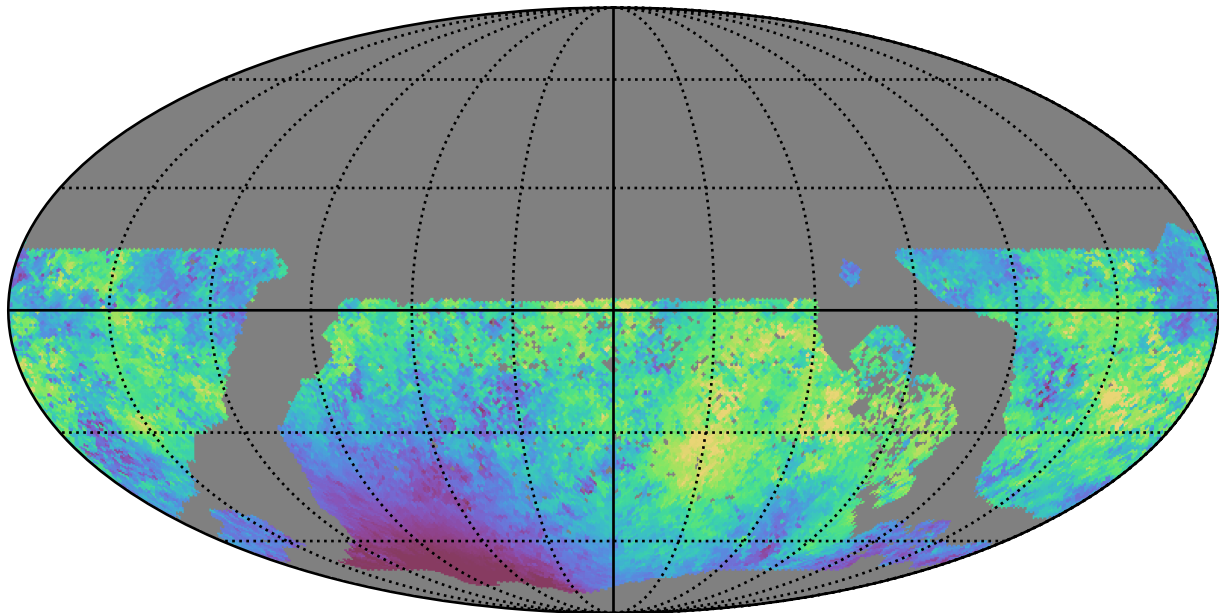
ddf_loaded_fl15_v3.4_10yrs WFD g band: Median moonDistance
