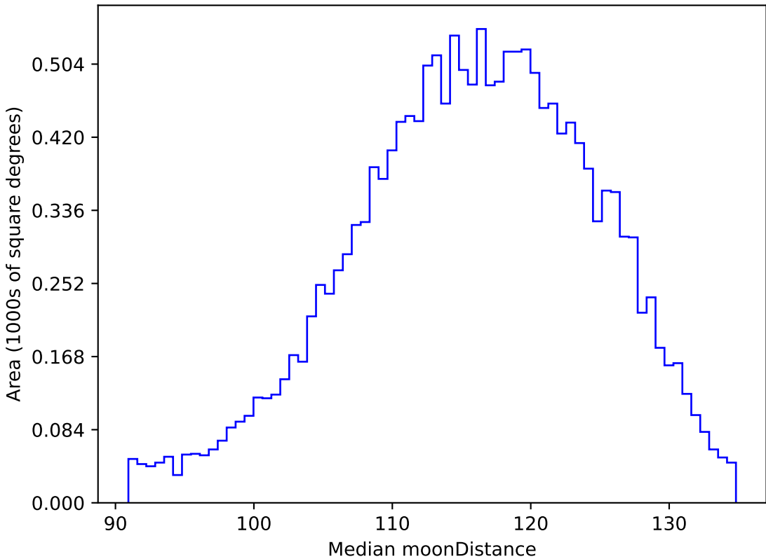
ddf_loaded_fl15_v3.4_10yrs WFD g band: Median moonDistance
