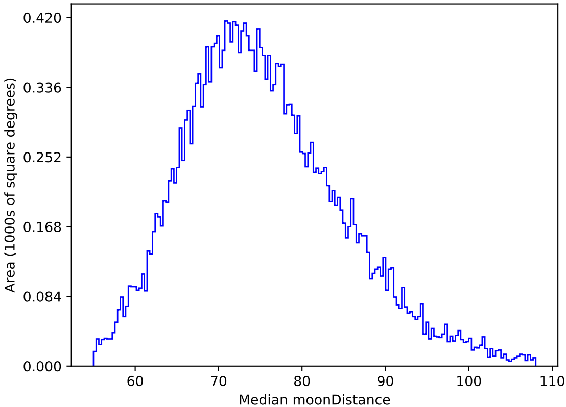
ddf_loaded_fl15_v3.4_10yrs All sky z band: Median moonDistance
