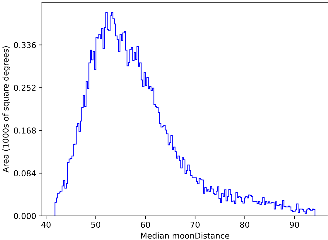
ddf_loaded_fl15_v3.4_10yrs All sky y band: Median moonDistance
