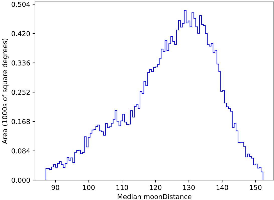
ddf_loaded_fl15_v3.4_10yrs All sky u band: Median moonDistance
