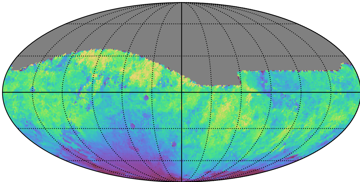
ddf_loaded_fl15_v3.4_10yrs All sky r band: Median moonDistance
