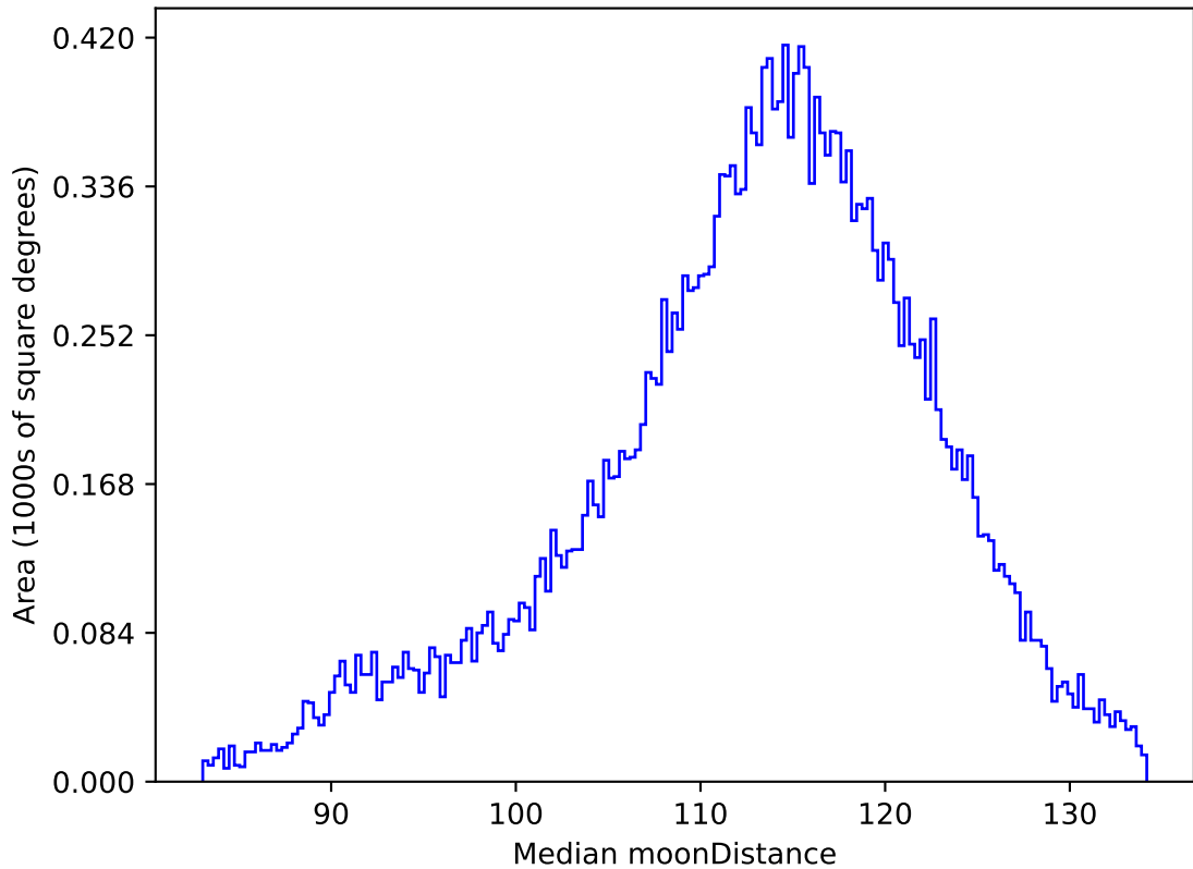
ddf_loaded_fl15_v3.4_10yrs All sky r band: Median moonDistance
