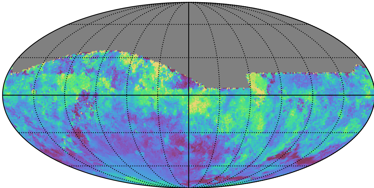
ddf_loaded_fl15_v3.4_10yrs All sky i band: Median moonDistance
