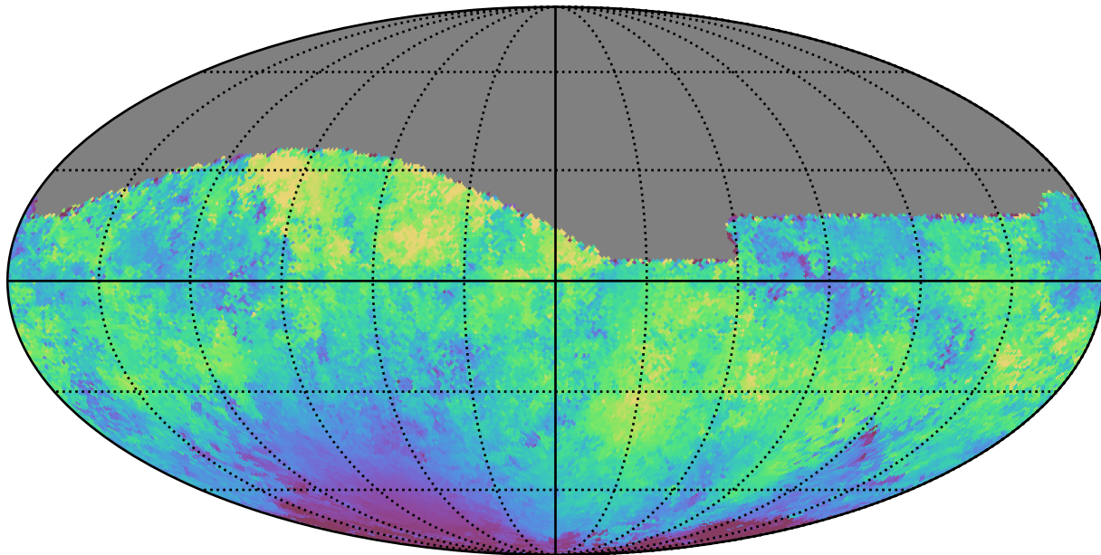
ddf_loaded_fl15_v3.4_10yrs All sky g band: Median moonDistance
