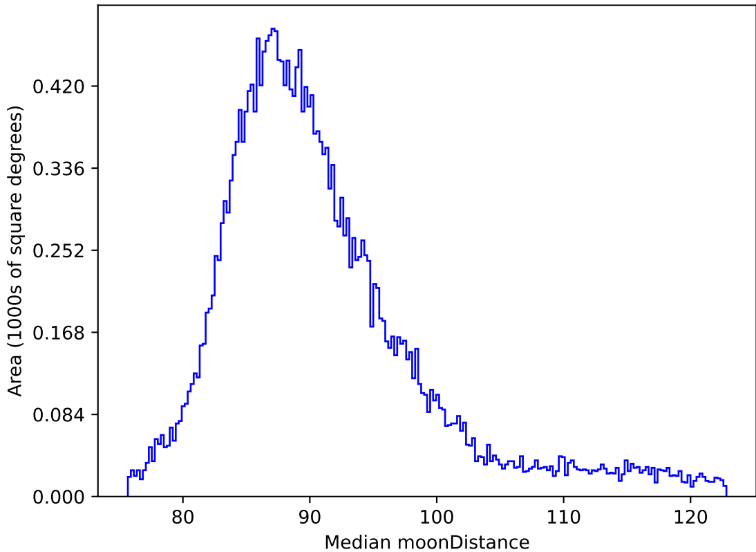
ddf_loaded_fl15_v3.4_10yrs All sky all bands: Median moonDistance
