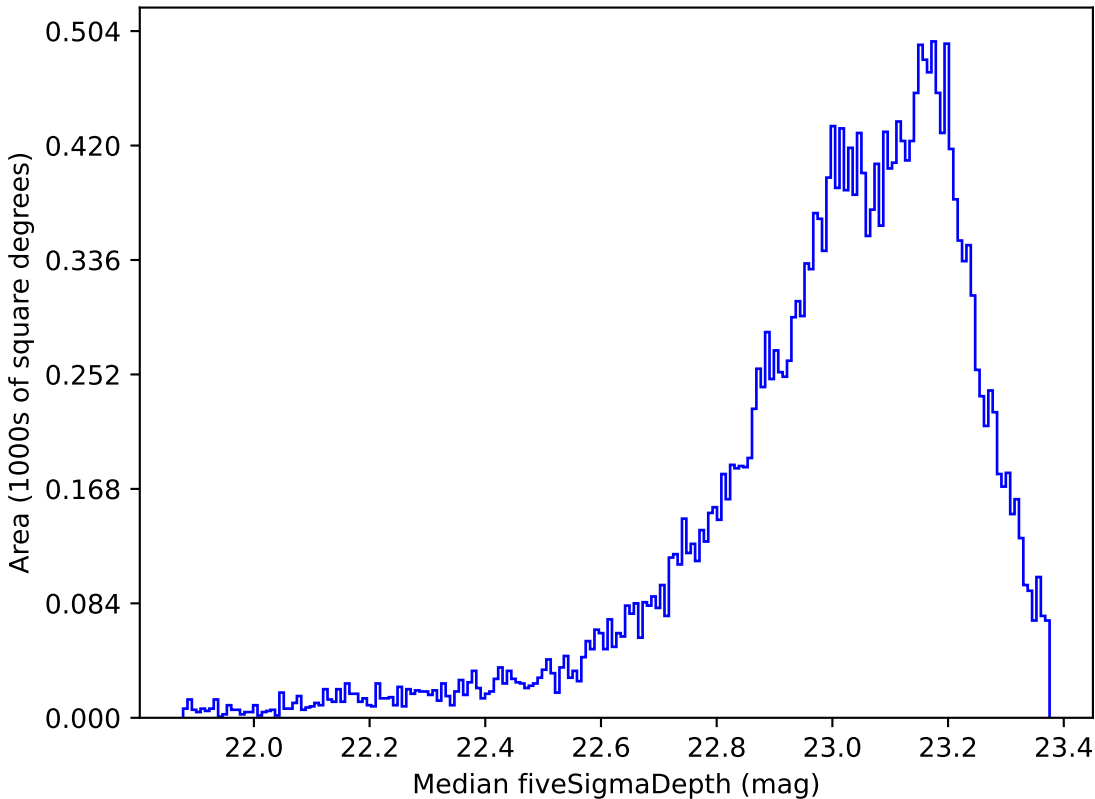
ddf_loaded_fl15_v3.4_10yrs Yr 1 z band: Median fiveSigmaDepth
