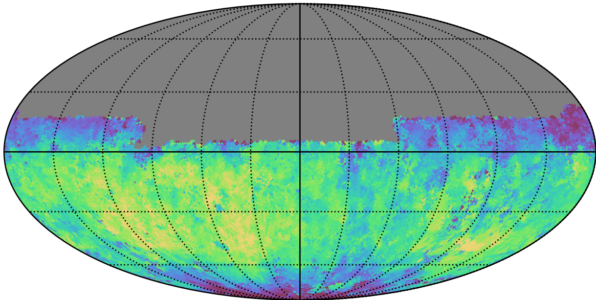
ddf_loaded_fl15_v3.4_10yrs Yr 1 y band: Median fiveSigmaDepth
