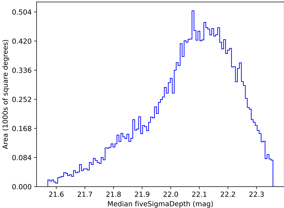
ddf_loaded_fl15_v3.4_10yrs Yr 1 y band: Median fiveSigmaDepth
