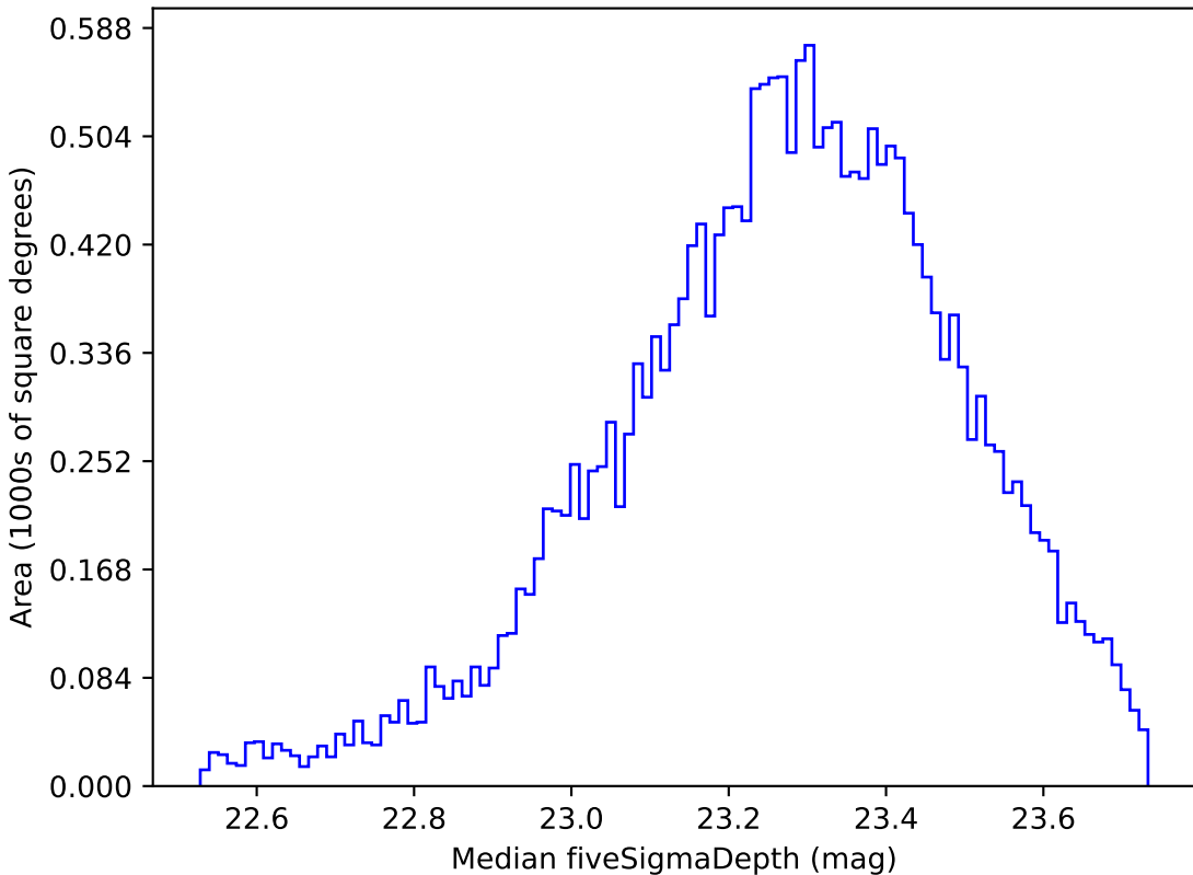
ddf_loaded_fl15_v3.4_10yrs Yr 1 u band: Median fiveSigmaDepth
