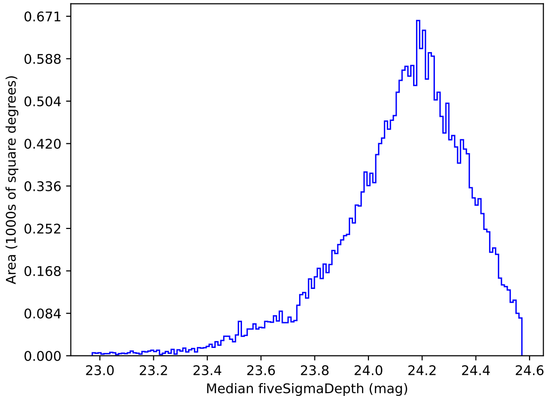
ddf_loaded_fl15_v3.4_10yrs Yr 1 r band: Median fiveSigmaDepth
