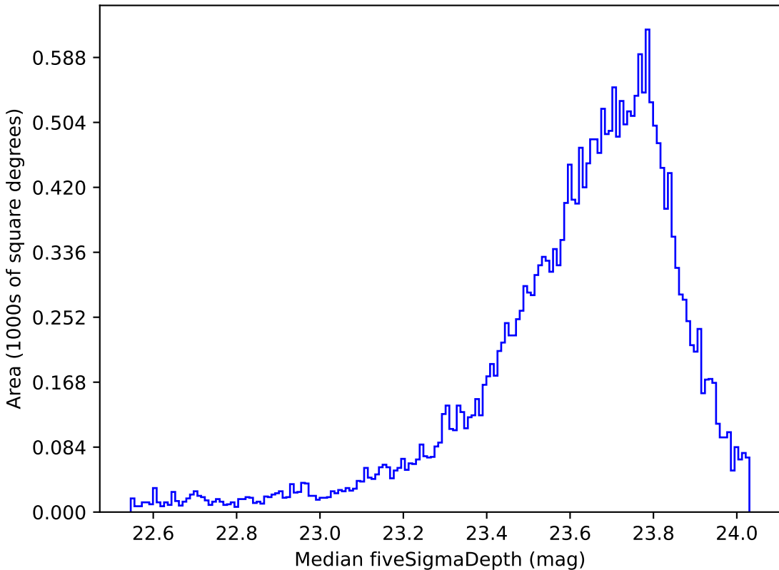
ddf_loaded_fl15_v3.4_10yrs Yr 1 i band: Median fiveSigmaDepth
