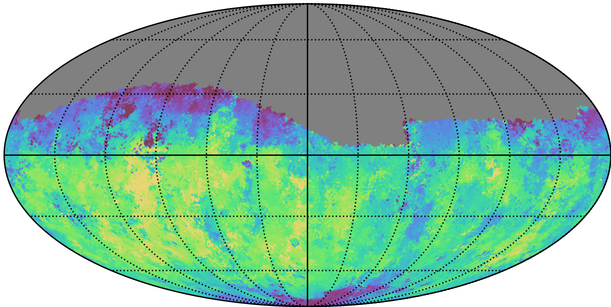
ddf_loaded_fl15_v3.4_10yrs Yr 1 g band: Median fiveSigmaDepth
