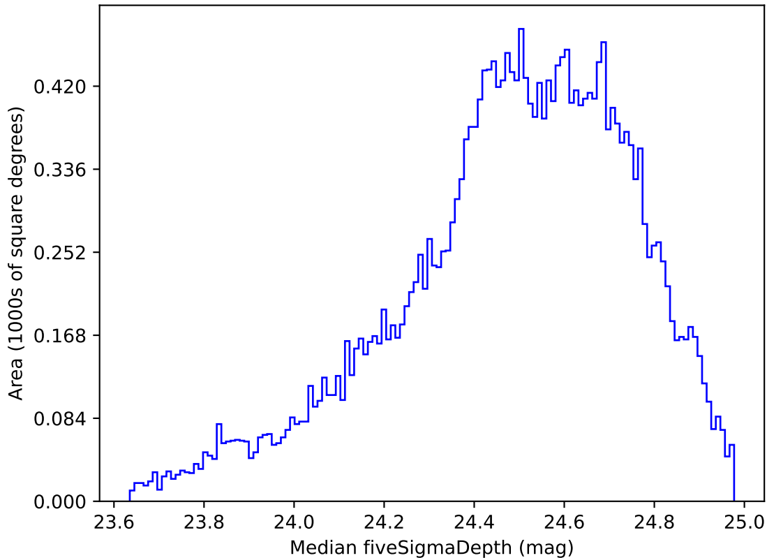
ddf_loaded_fl15_v3.4_10yrs Yr 1 g band: Median fiveSigmaDepth
