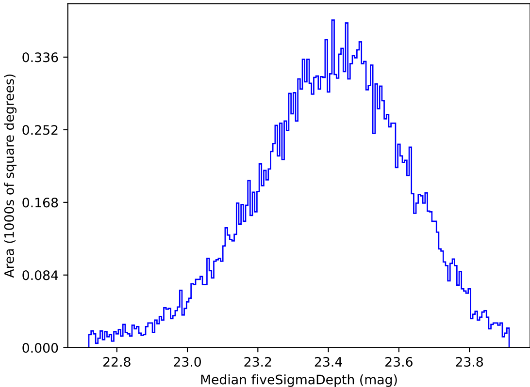
ddf_loaded_fl15_v3.4_10yrs Yr 1 all bands: Median fiveSigmaDepth
