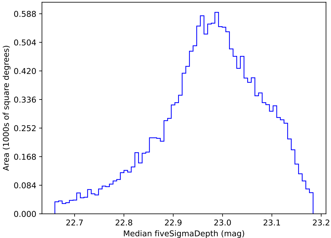
ddf_loaded_fl15_v3.4_10yrs WFD z band: Median fiveSigmaDepth
