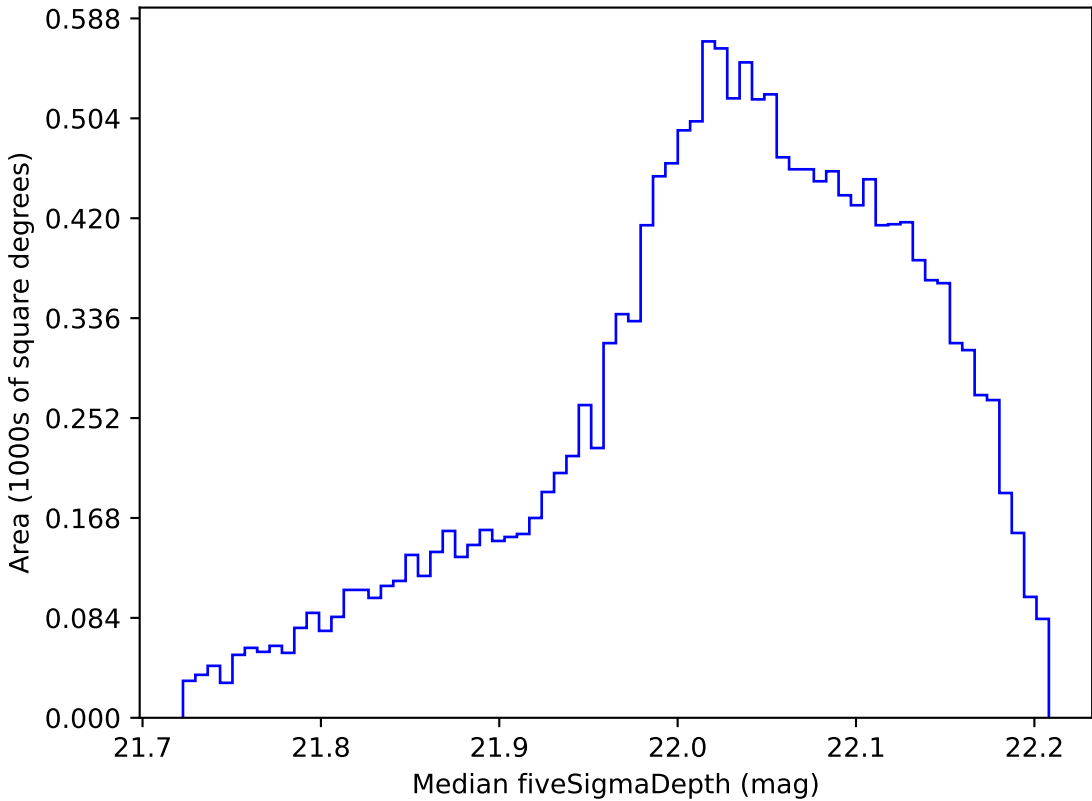
ddf_loaded_fl15_v3.4_10yrs WFD y band: Median fiveSigmaDepth
