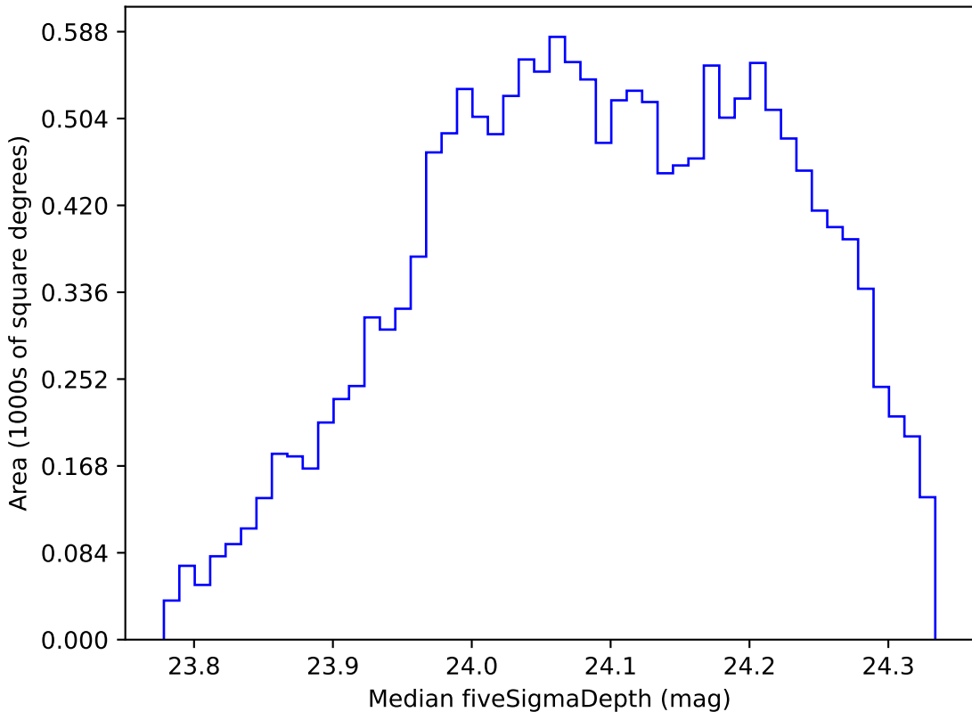
ddf_loaded_fl15_v3.4_10yrs WFD r band: Median fiveSigmaDepth
