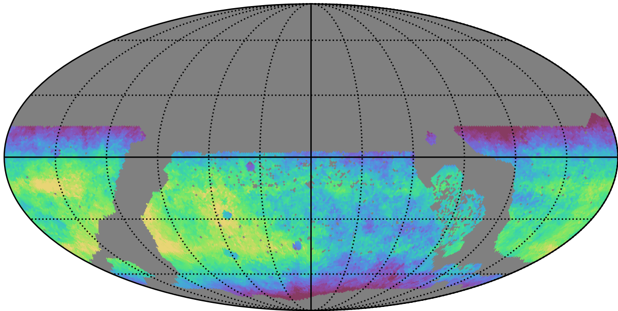
ddf_loaded_fl15_v3.4_10yrs WFD i band: Median fiveSigmaDepth
