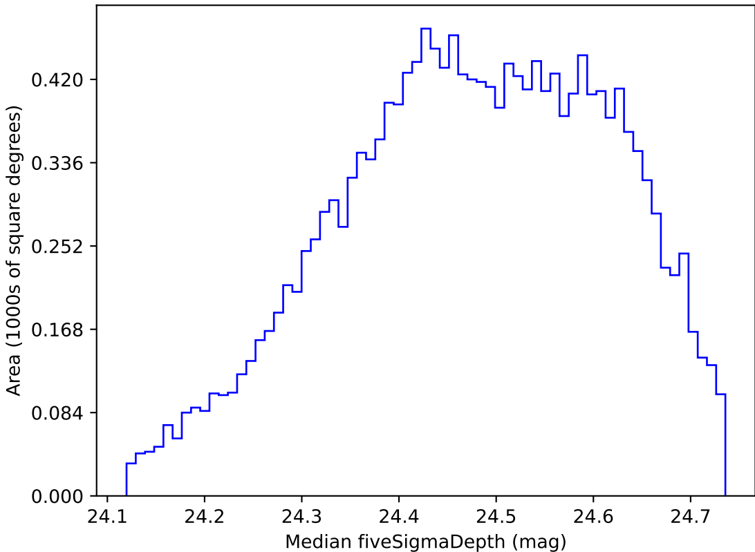
ddf_loaded_fl15_v3.4_10yrs WFD g band: Median fiveSigmaDepth
