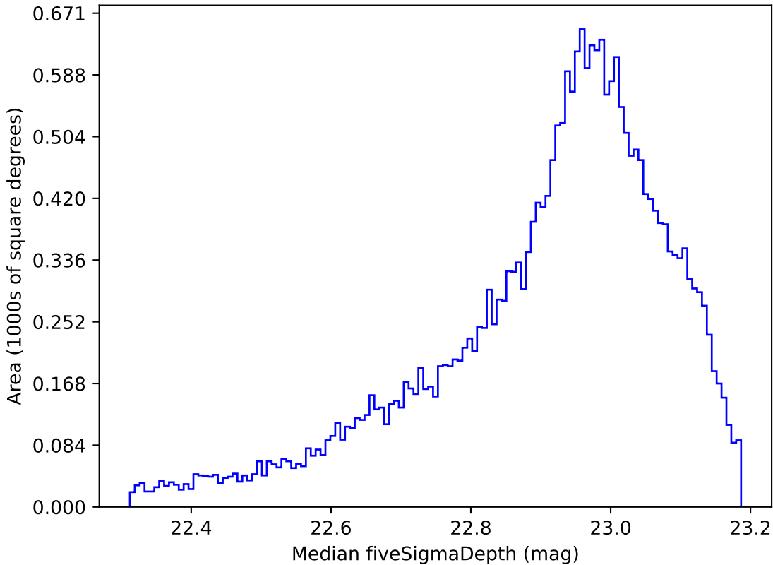
ddf_loaded_fl15_v3.4_10yrs All sky z band: Median fiveSigmaDepth
