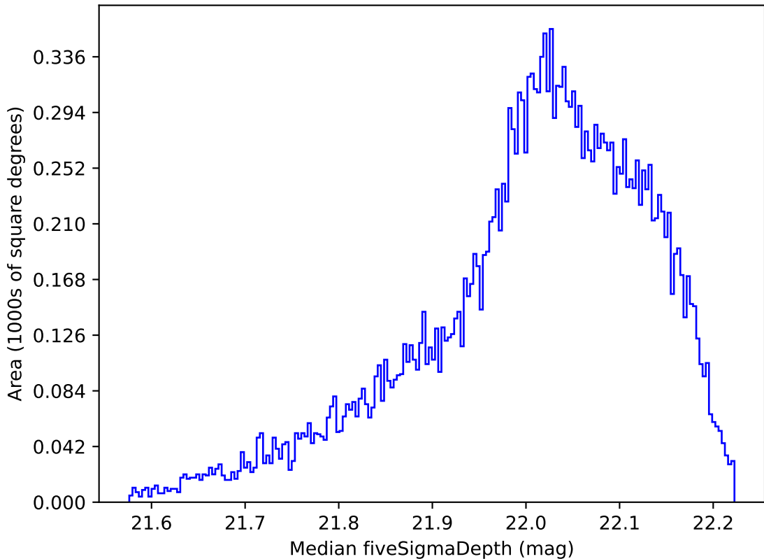
ddf_loaded_fl15_v3.4_10yrs All sky y band: Median fiveSigmaDepth
