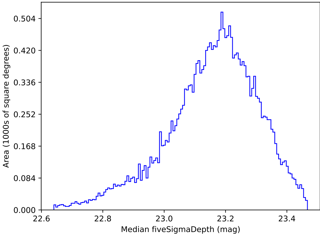
ddf_loaded_fl15_v3.4_10yrs All sky u band: Median fiveSigmaDepth
