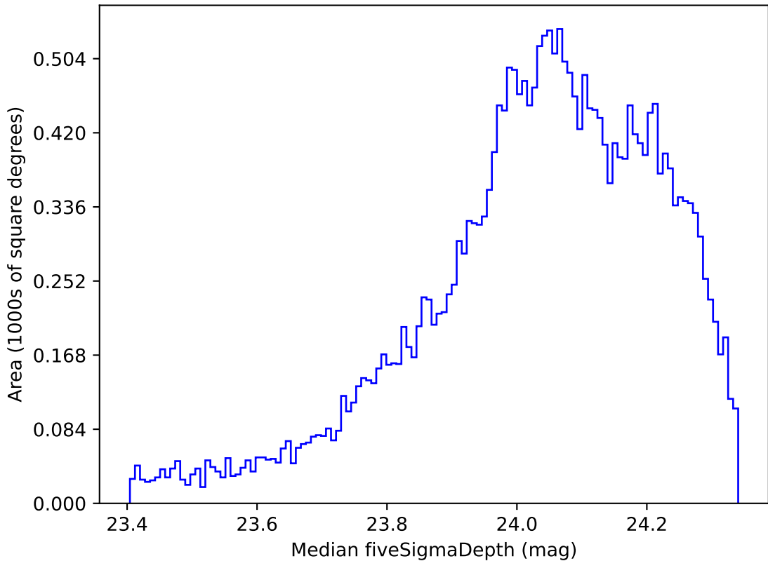
ddf_loaded_fl15_v3.4_10yrs All sky r band: Median fiveSigmaDepth
