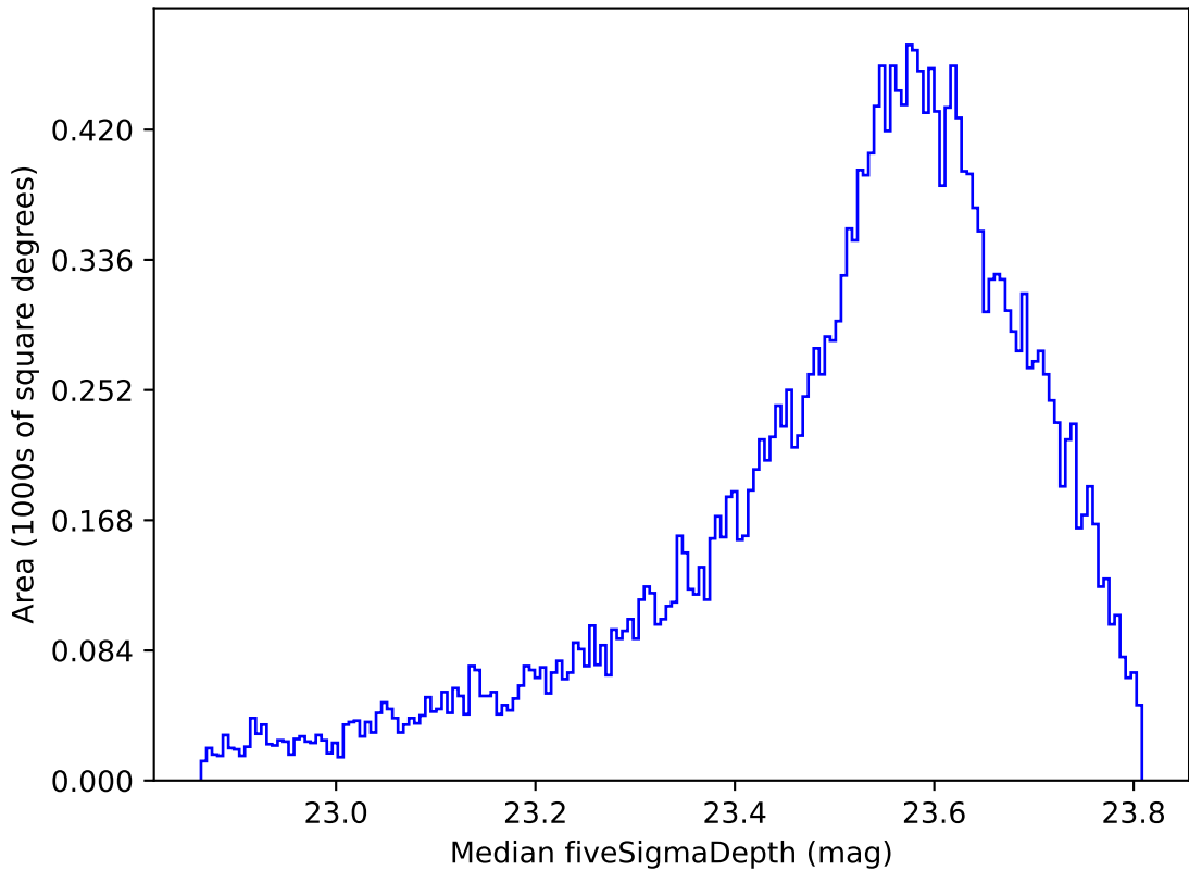
ddf_loaded_fl15_v3.4_10yrs All sky i band: Median fiveSigmaDepth
