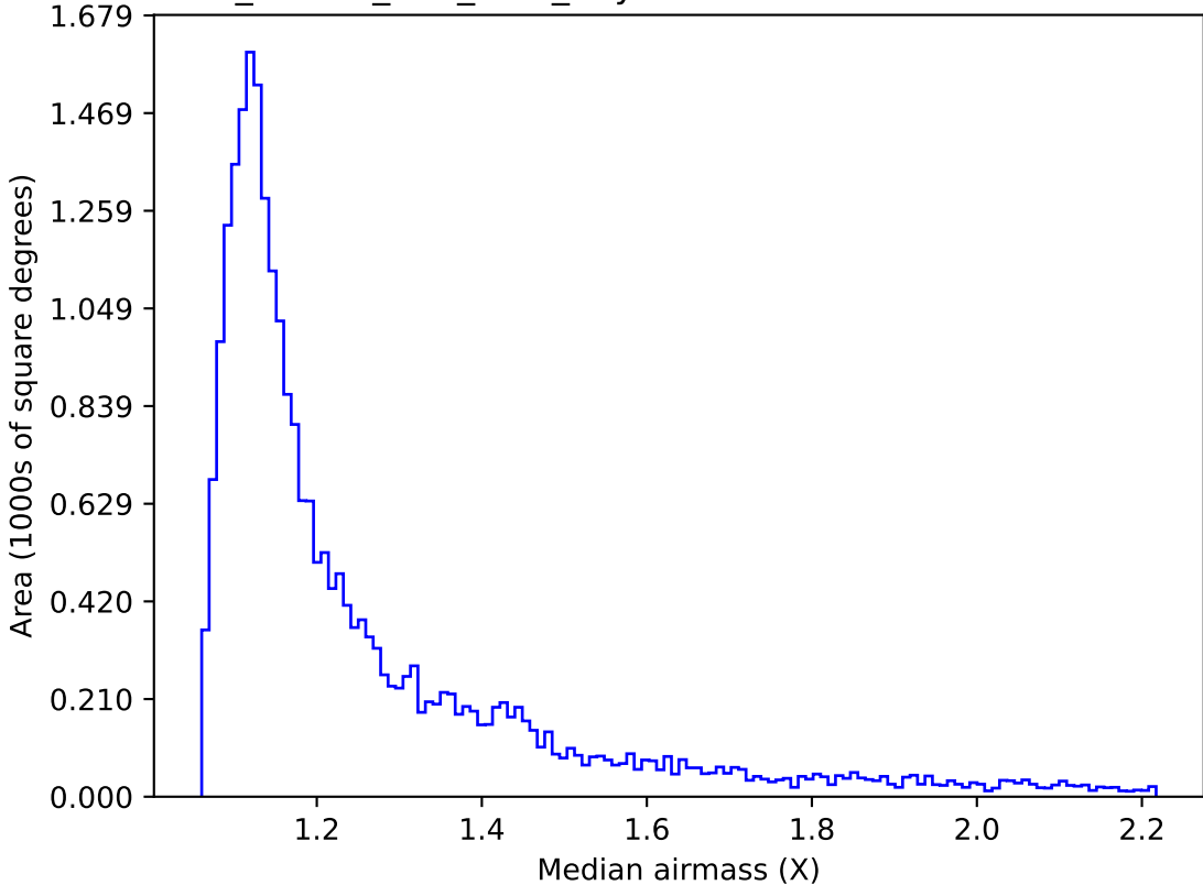
ddf_loaded_fl15_v3.4_10yrs Yr 1 z band: Median airmass
