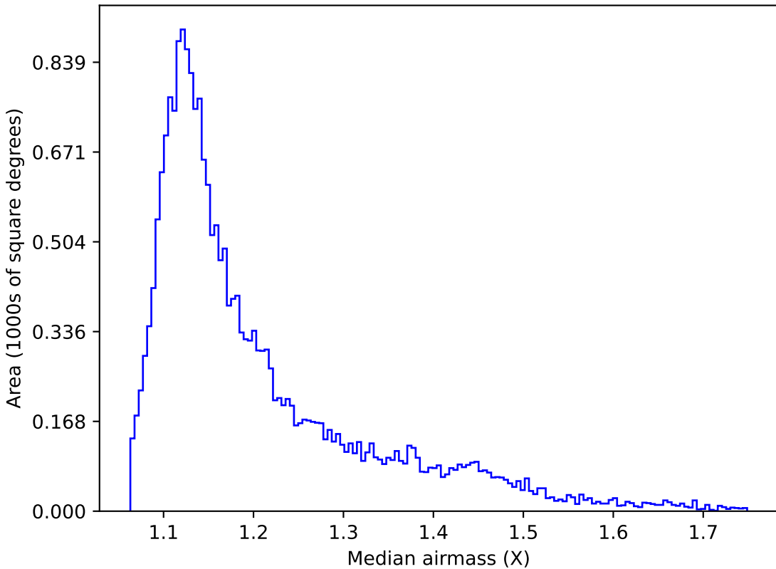
ddf_loaded_fl15_v3.4_10yrs Yr 1 y band: Median airmass
