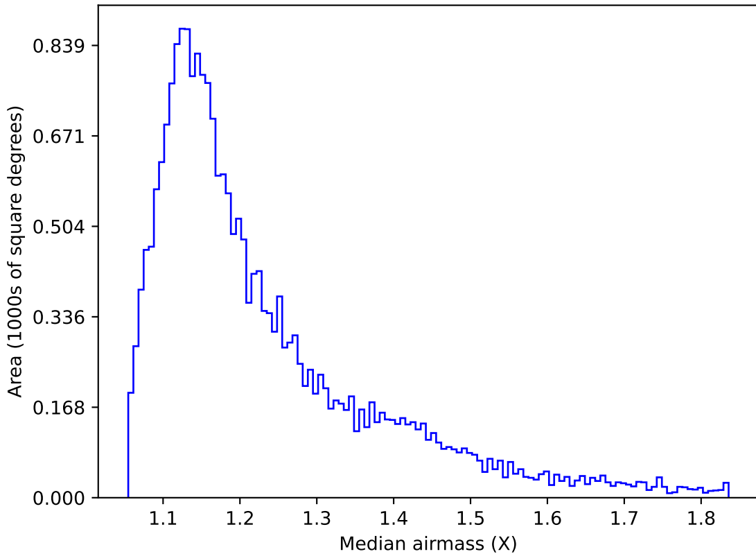
ddf_loaded_fl15_v3.4_10yrs Yr 1 u band: Median airmass
