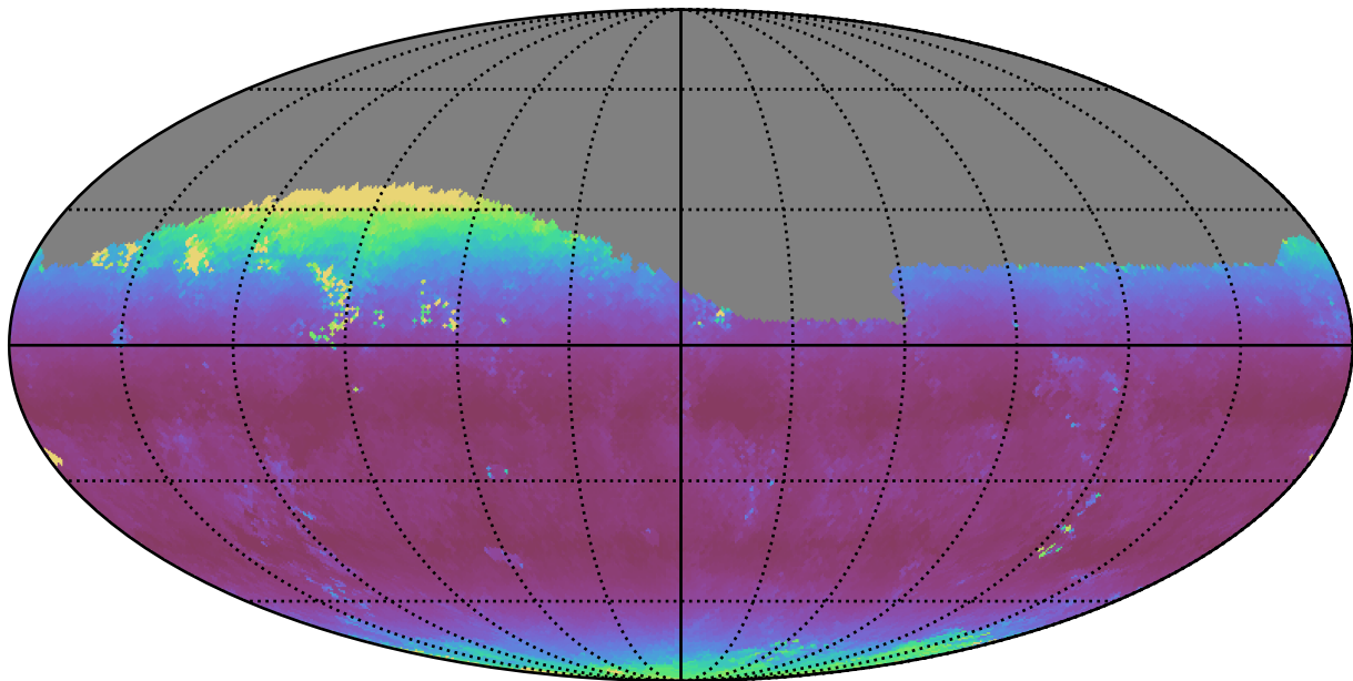
ddf_loaded_fl15_v3.4_10yrs Yr 1 i band: Median airmass
