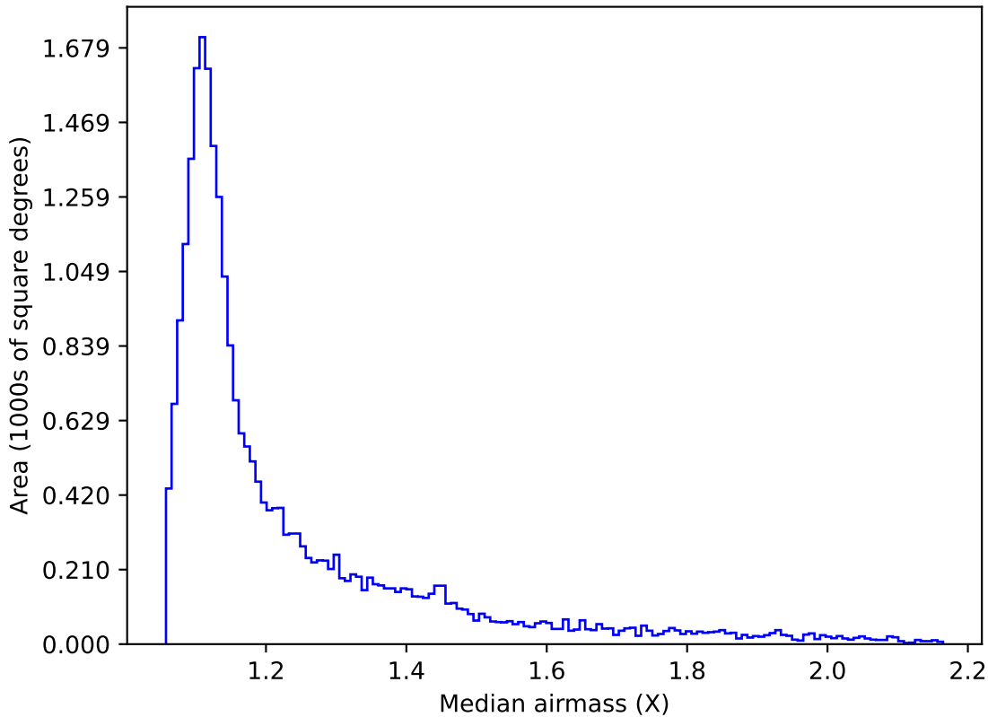
ddf_loaded_fl15_v3.4_10yrs Yr 1 i band: Median airmass
