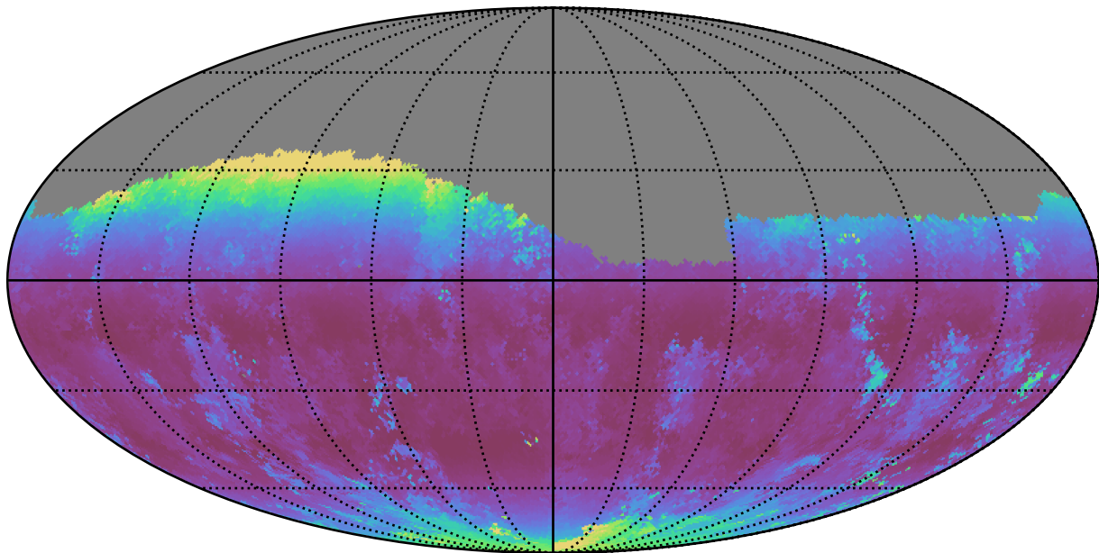
ddf_loaded_fl15_v3.4_10yrs Yr 1 g band: Median airmass
