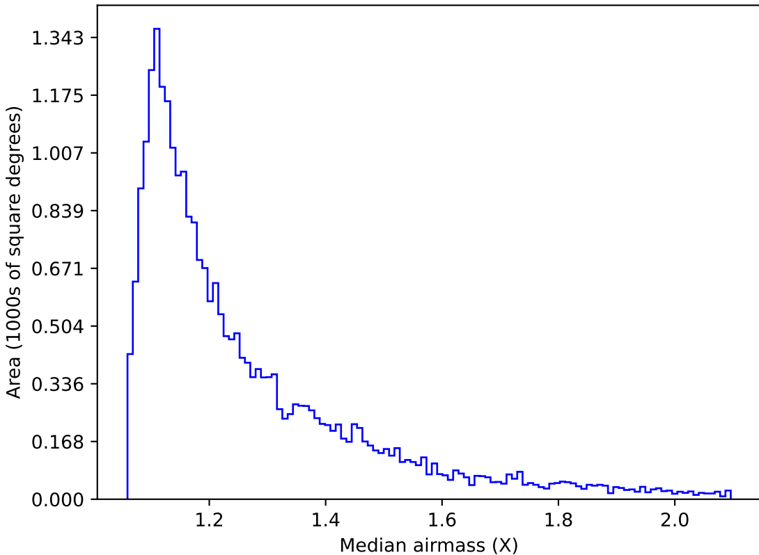
ddf_loaded_fl15_v3.4_10yrs Yr 1 g band: Median airmass
