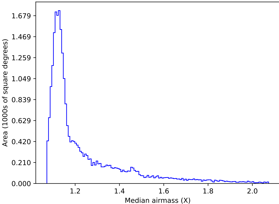
ddf_loaded_fl15_v3.4_10yrs Yr 1 all bands: Median airmass
