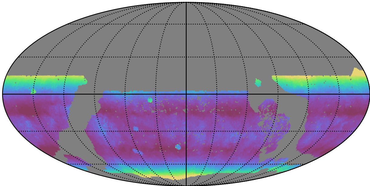
ddf_loaded_fl15_v3.4_10yrs WFD z band: Median airmass
