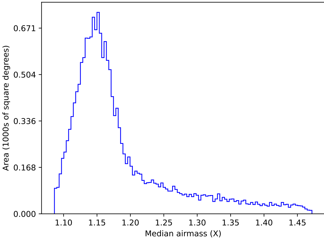
ddf_loaded_fl15_v3.4_10yrs WFD z band: Median airmass
