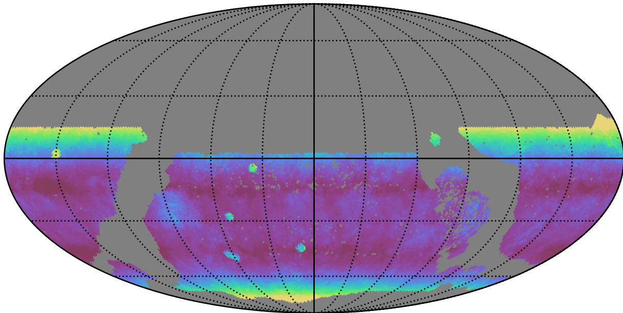
ddf_loaded_fl15_v3.4_10yrs WFD y band: Median airmass
