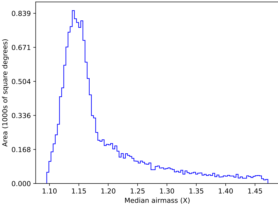
ddf_loaded_fl15_v3.4_10yrs WFD y band: Median airmass
